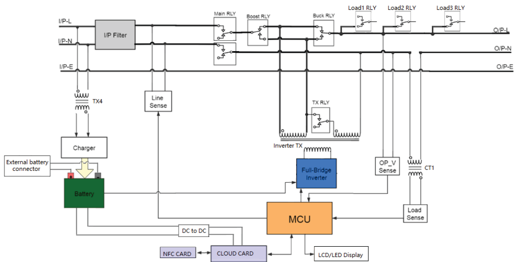
Figure 2. Block Diagram SMART1500LDCXNC
